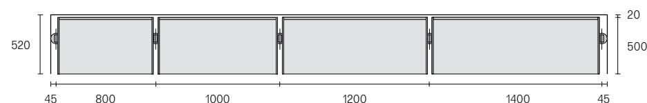
Ingombri composizione lineare con cassetteria e mensolone tv/HiFi Encumbrance of the linear composition with drawer unit and tv/HiFi top shelf holder
